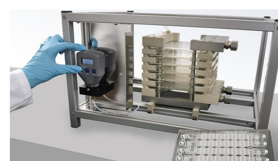
Microreactors
